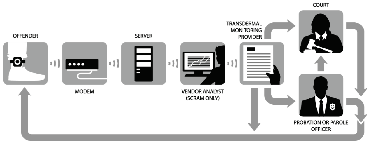
Figure 3 - Information Flow
